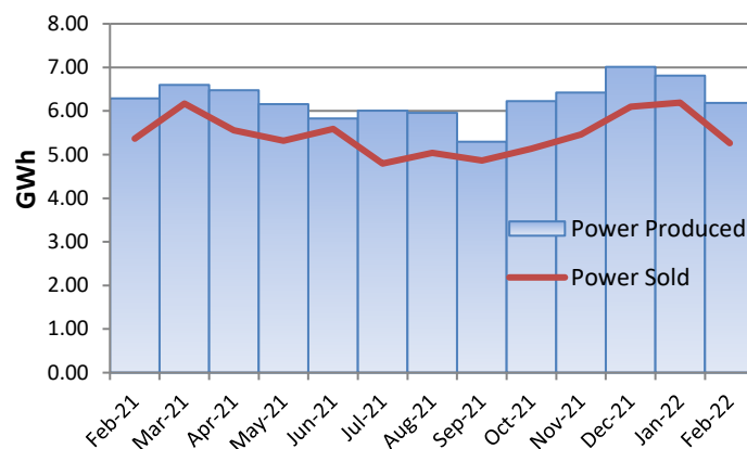
Figure 5: Electricity Generated and Sold
