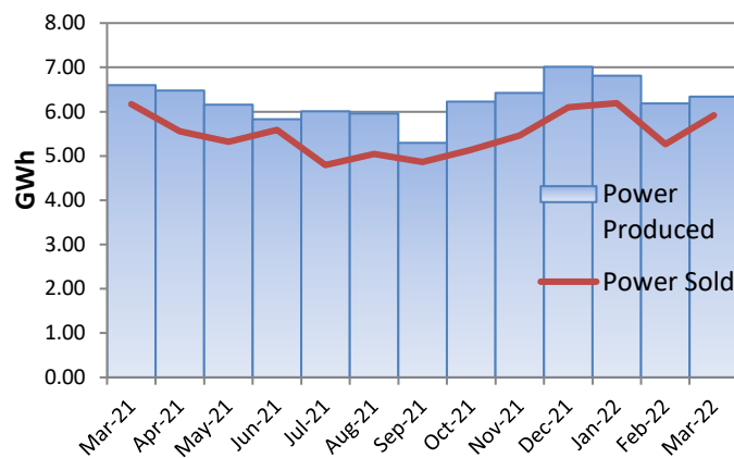
Figure 5: Electricity Generated and Sold
